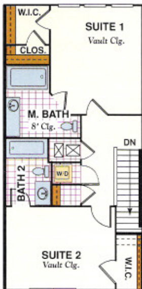
SECOND FLOOR PLAN INTERIOR UNIT PLAN
