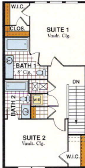
SECOND FLOOR PLAN END UNIT FLOOR PLAN
